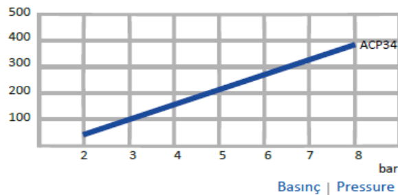
Tork | Torque Nm
